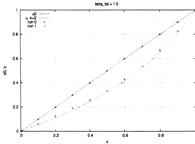
Figure 1: Primal solution during adaptation for \beta_{\text{tol}}=1 ( k=2 ).
